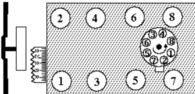
Figure 1- Pontiac 389-455 c.i.d. V8 Firing Order 1-8-4-3-6-5-7-2 Turn distributor clockwise to advance timing.
