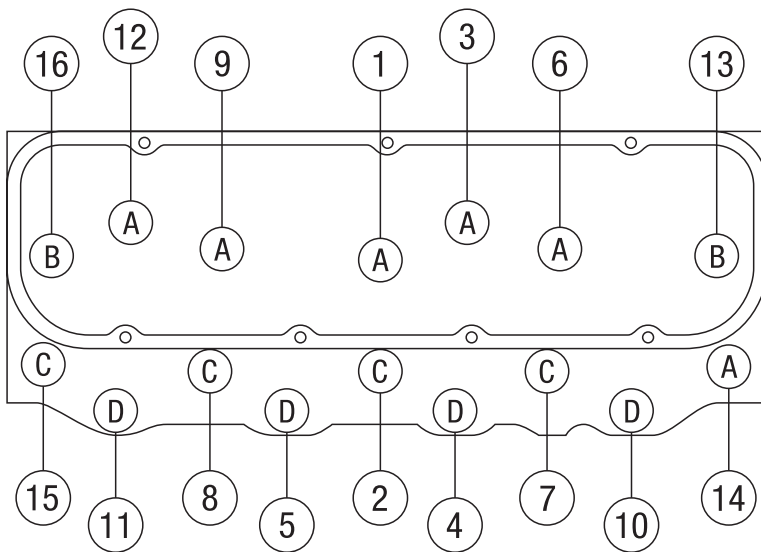
Figure 1 - Big Block Chevrolet Cylinder Head Bolt Torque Sequence
