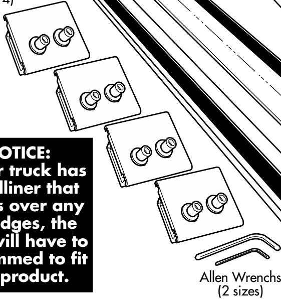
Rail Clamp Assemblies (x 4)
