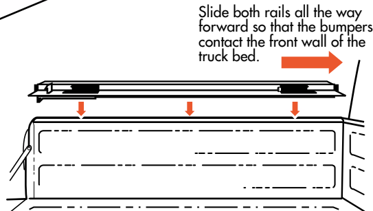
Position Side Rails on side walls of truck bed. Spring blocks go toward the cab. Locking catch goes on left side toward the tailgate as shown.
