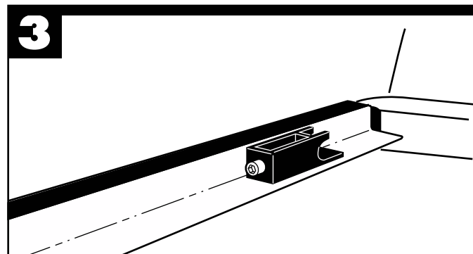
Slide both rails all the way forward so that the bumpers contact the front wall of the truck bed.
