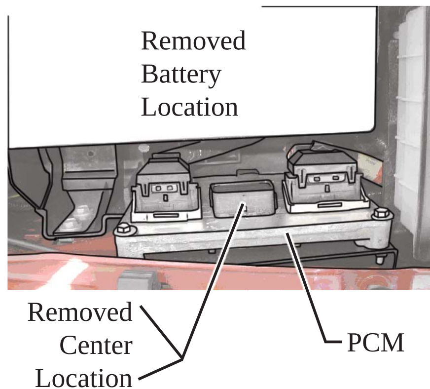
FIGURE 2 - PCM Location
