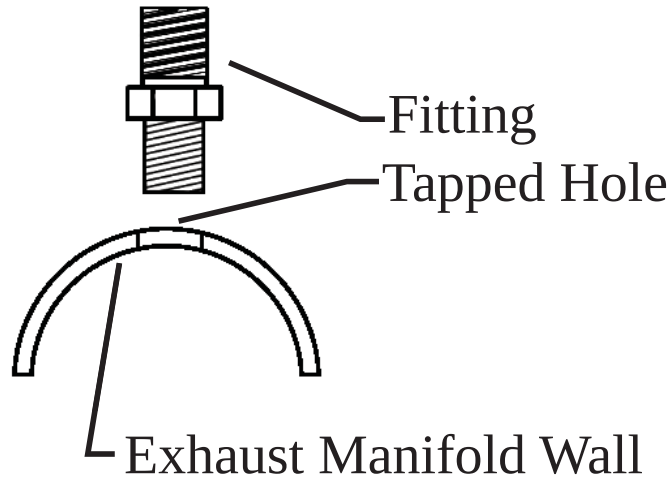
Figure 1 - Fitting Installation
