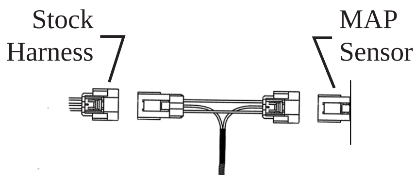
FIGURE 2 - "T" ASSEMBLY
