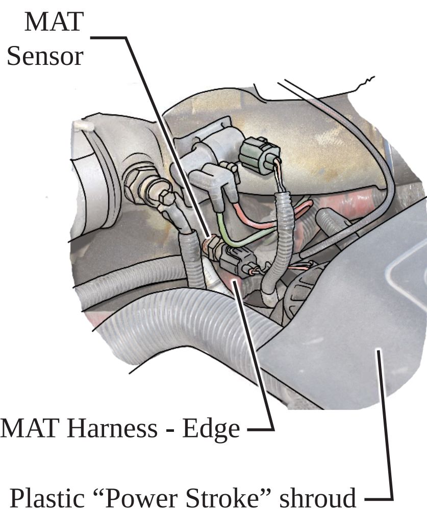
FIGURE 5 - ASSEMBLED VIEW
