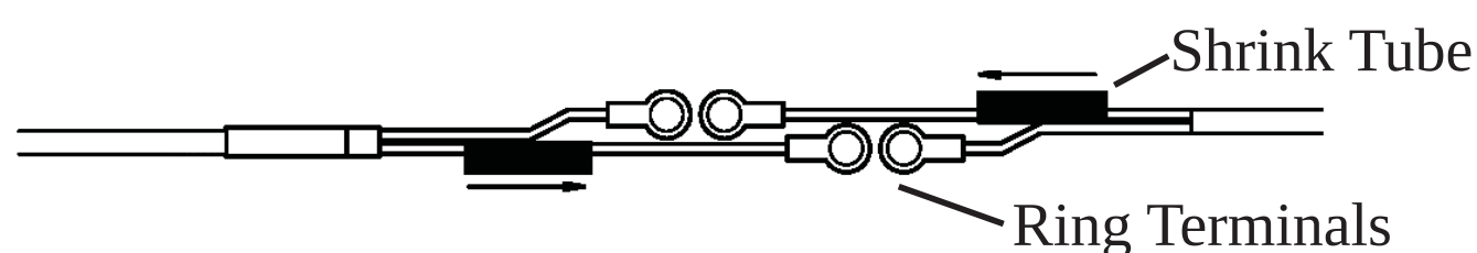
Figure 5 - Shrink Tube
