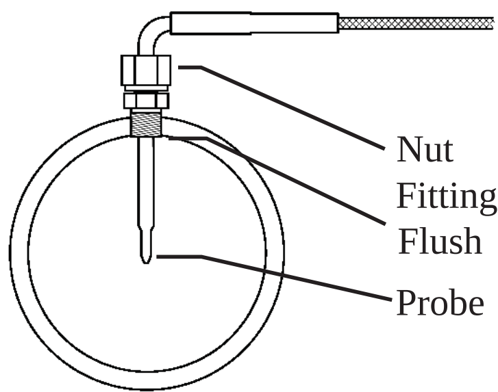
Figure 2 - Probe Insertion
