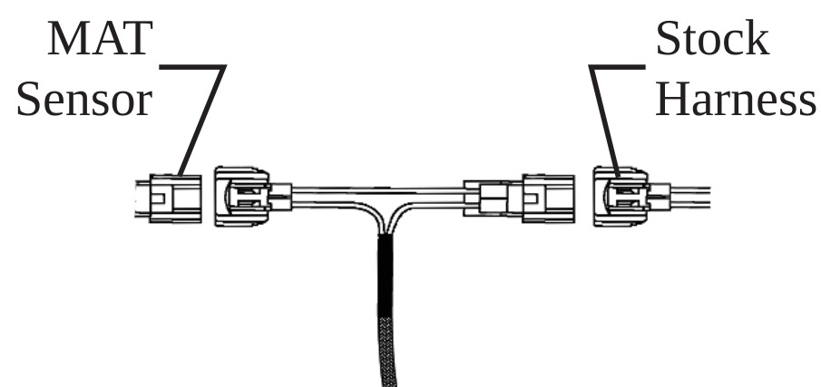
FIGURE 4 - "T" ASSEMBLY
