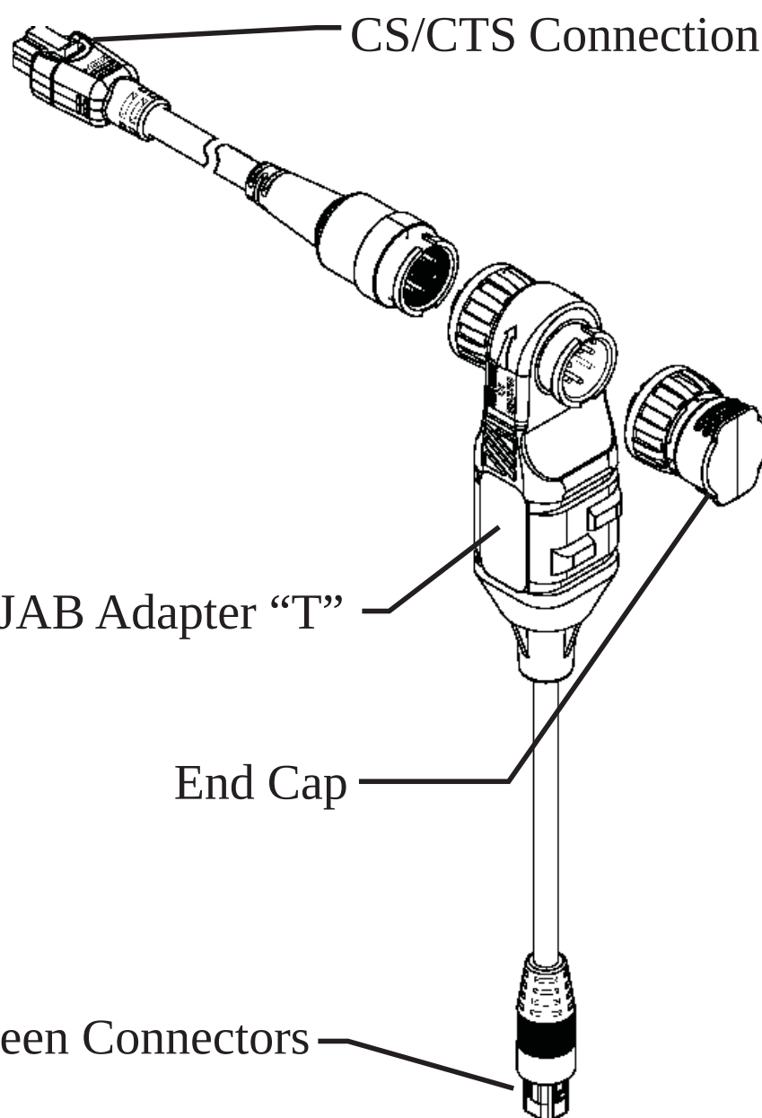
Figure 2 - JAB System
