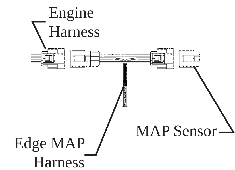
FIGURE 6 - "T" Assembly
