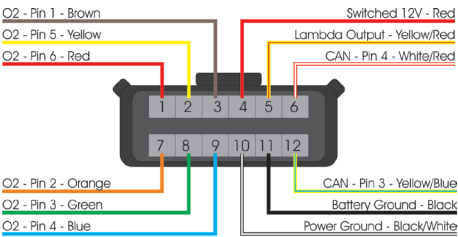
Harness Connector Rear View
