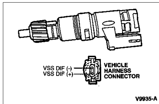
CONNECTOR FACE (Looking INTO Connector)
