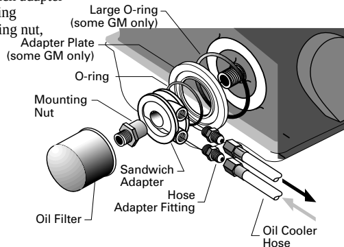
FIGURE 3 Sandwich Adapter Installation
