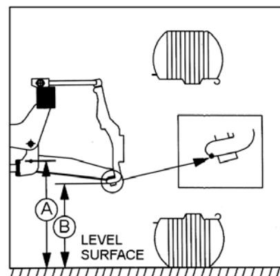
DIAGRAM 10 - Ride height adjustment.
