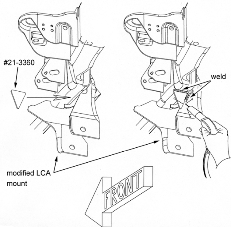
DIAGRAM 7 - WELDING THE #21-3360 GUSSETS - Position where shown, weld to frame and LCA mount on driver and passenger side. Driver side shown.
