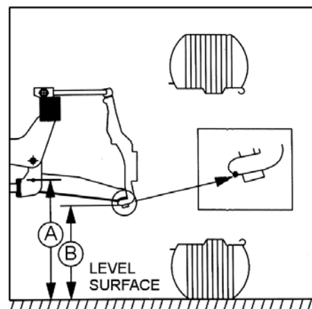
DIAGRAM 15 - Ride height adjustment.
