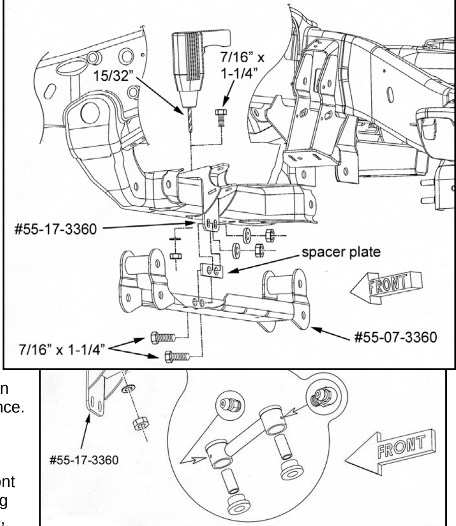
DIAGRAM 10 - INSTALLING THE #55-07-3360 FRONT CROSSMEMBER AND #55-17-3360 C.S.S. MOUNTING BRACKET.
