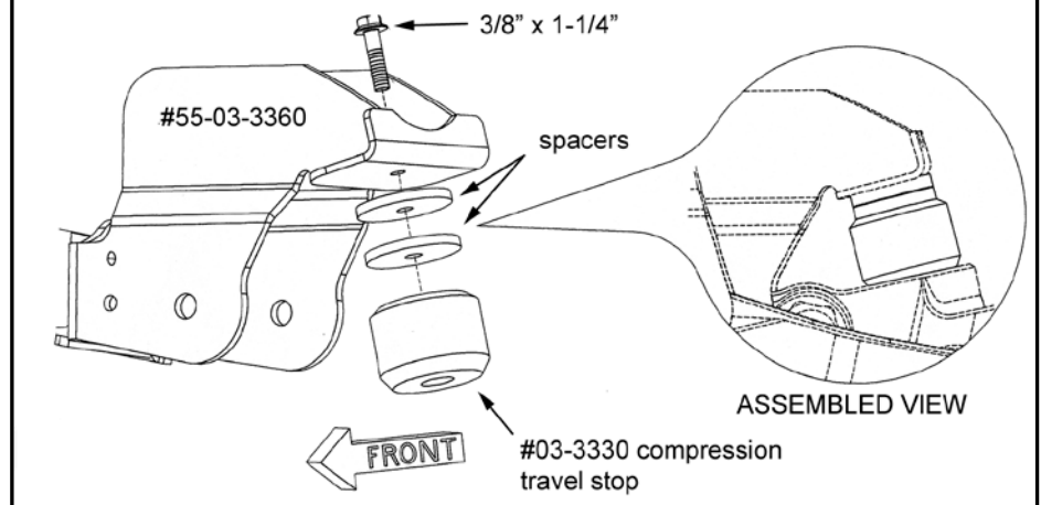
DIAGRAM 13 - #03-3330 COMPRESSION TRAVEL STOPS - Determine the necessary number of spacers, if any, to use, then install as indicated.
