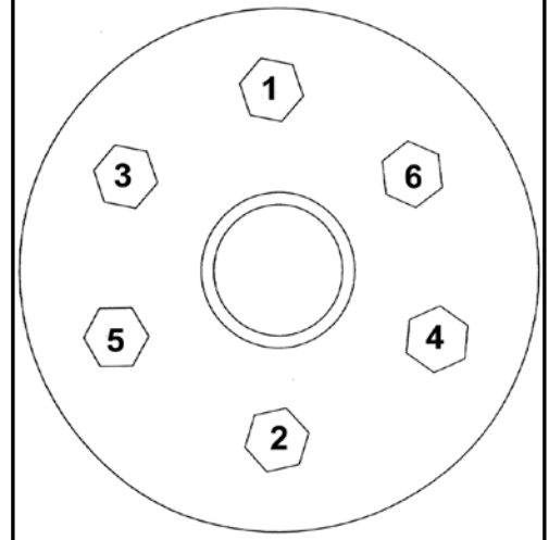
DIAGRAM 14- LUG NUT TORQUE SEQUENCE - Use the sequence shown to torque the lug nuts.
