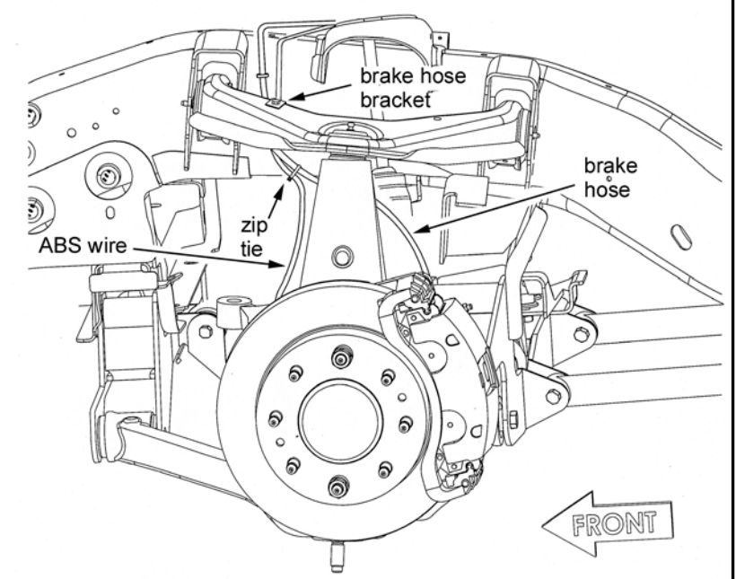
DIAGRAM 4B - BRAKE HOSE AND ABS ROUTING.
