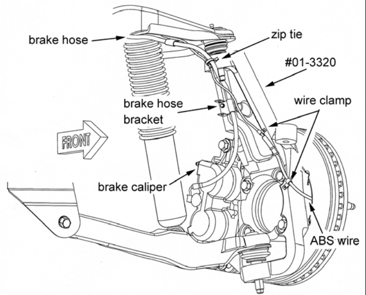
DIAGRAM 4A - BRAKE HOSE AND ABS WIRE ROUTING, REAR VIEW.
