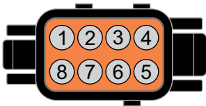
Transmission Breakout Connector DTM06-8S (Wire side view)
