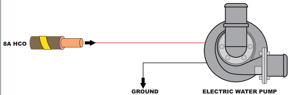
Example 8A HCO Wiring Connections
