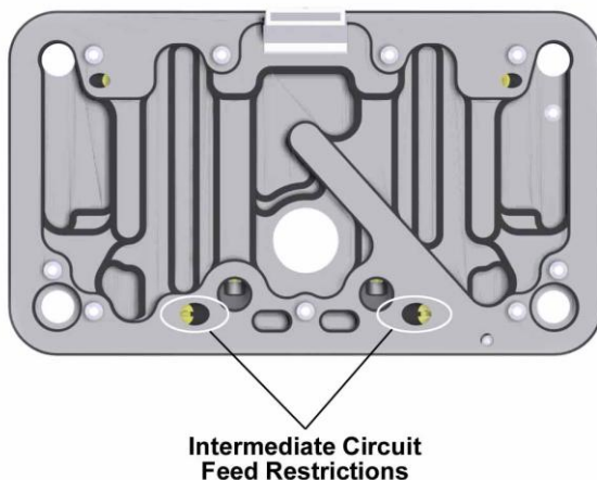
3 Circuit Billet Metering Block (Back) Model 4500 Ultra HP DOMINATOR Figure 8
