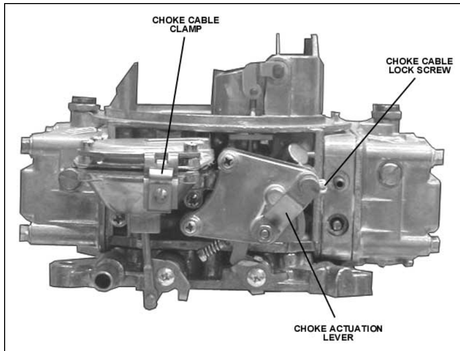
Figure 2b. Manual choke parts (0-81850 shown)
