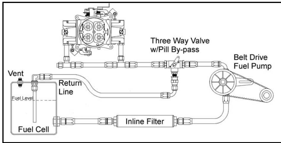
Belt Drive Fuel Pump with Three-Way Safety Valve
