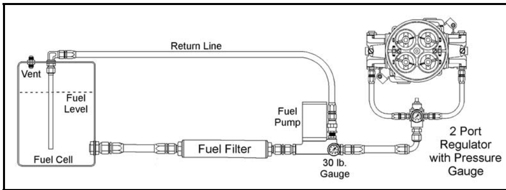
Single Carburetor with 350/500 GPH Holley Dominator Fuel Pump
