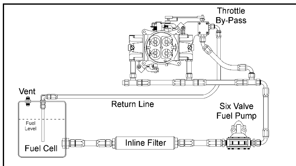
Throttle By-Pass System with Six Valve Fuel Pump
