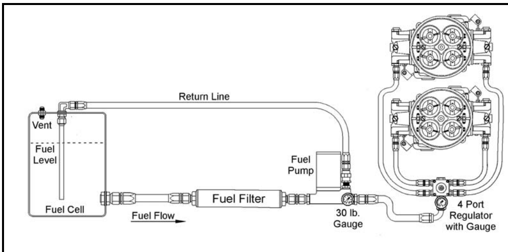
Dual Carburetor with 500 GPH Holley Dominator Fuel Pump
