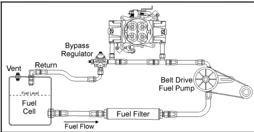
Belt Drive Fuel Pump with Bypass Regulator
