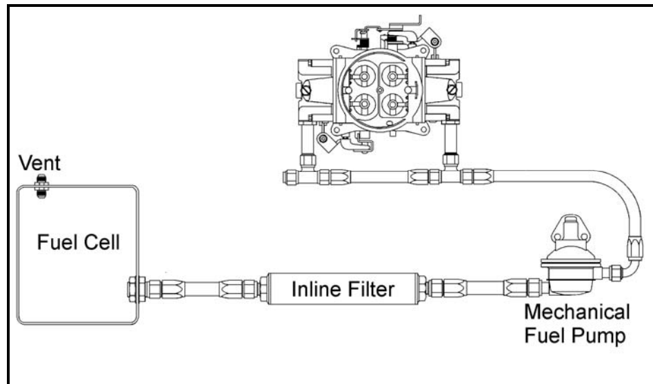
Hi-Flow Mechanical Fuel Pump system
