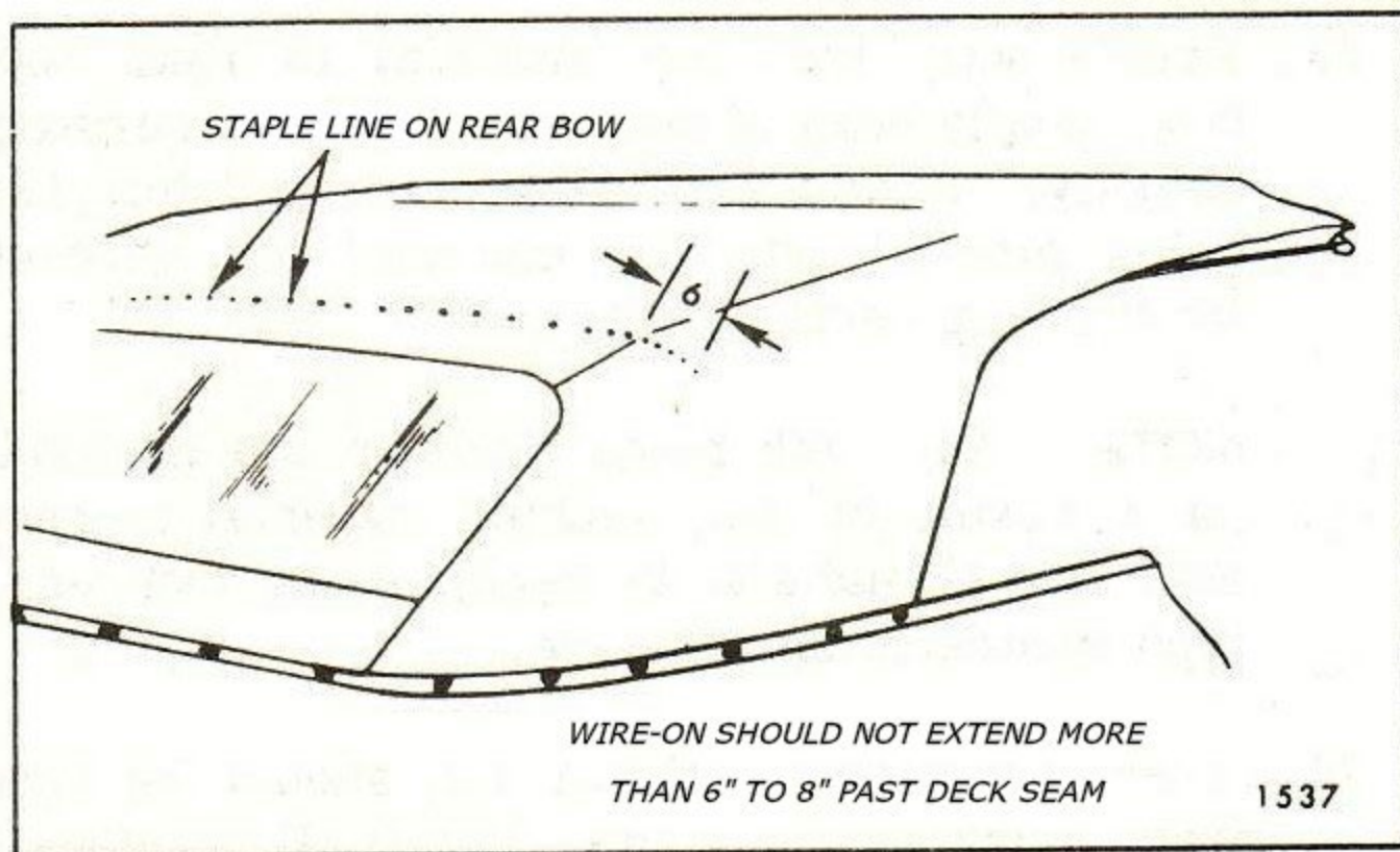
Fig. 13-42 — Tacking Outboard of Seams
