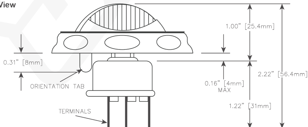
MFA134 – 4 Position Switch (Actual Size)
