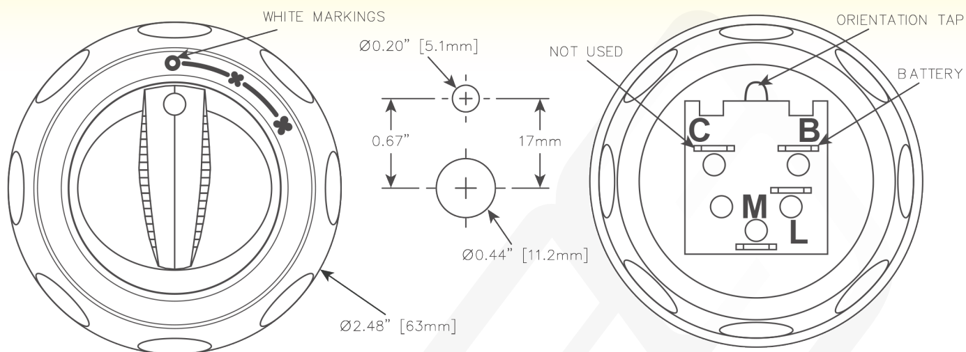
MFA133 – 3 Position Switch (Actual Size)
