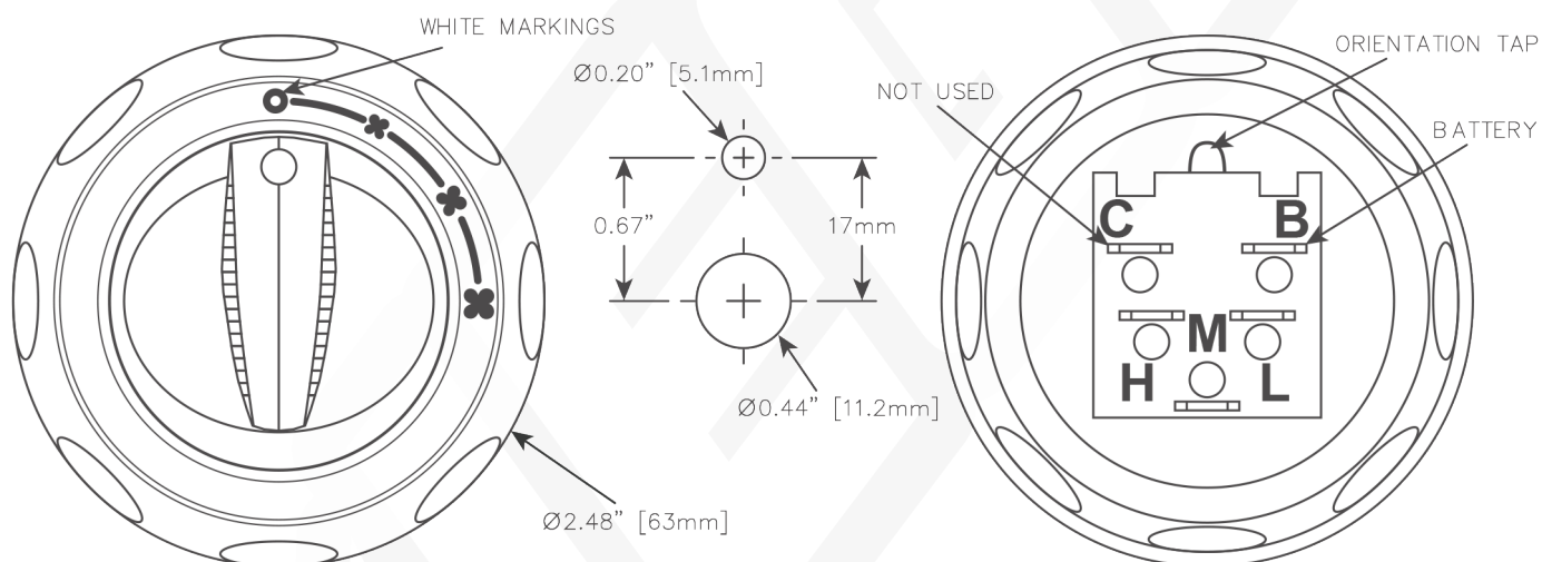
MFA134 – 4 Position Switch (Actual Size)
