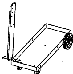
Figure C: Connection of Bottom Shelf and Left Support
