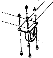
Figure B: Caster Attachment
