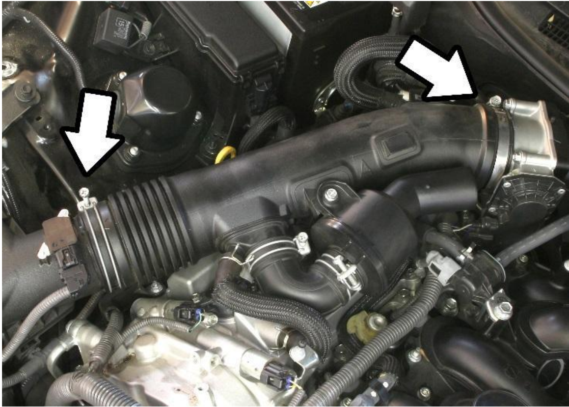
5. Loosen the hose clamps on the throttle body and air box.
