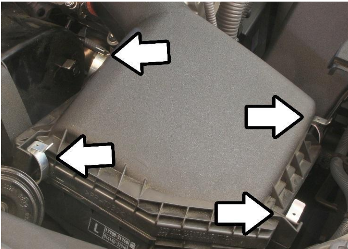
6. Unclip the four buckles securing the upper air box.
