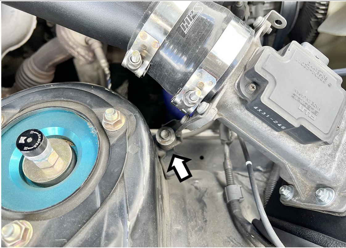
23. Reinstall the MAF sensor mounting bolt.
