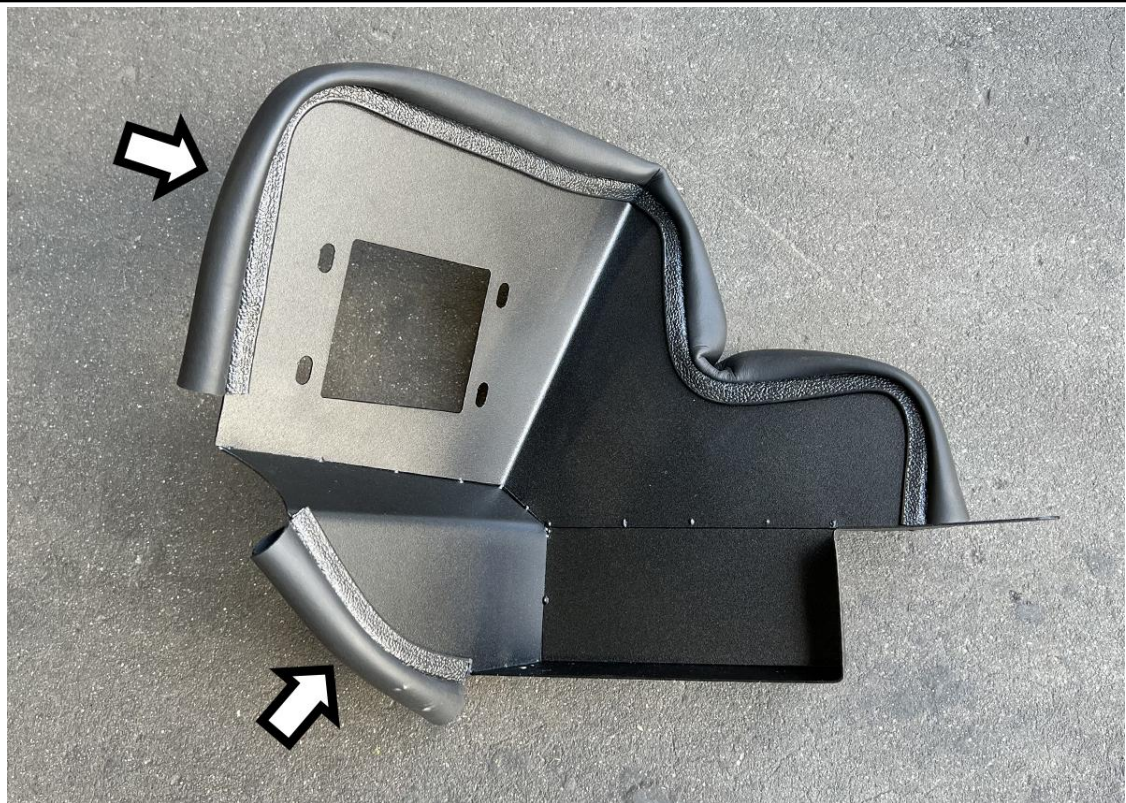
12. Install the provided bubble edge trim onto the heat shield as shown.
