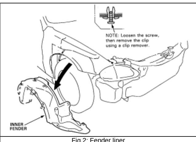
Fig.2: Fender liner
