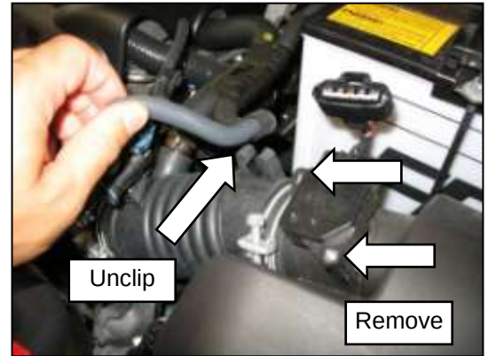
b. Unplug the Mass Air Flow (MAF) sensor wire connector. Loosen the two screws securing the MAF sensor and carefully remove the sensor. Unclip the EVAP VSV hose from the intake tube.
