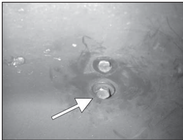
f. From inside the passenger side wheel well, remove the bolt holding the air box base in place.
