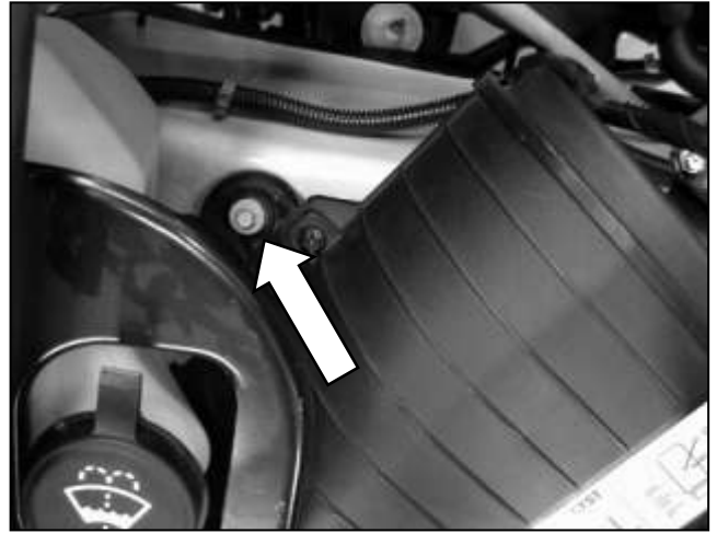
f. Loosen the third bolt holding in the stock air box.
