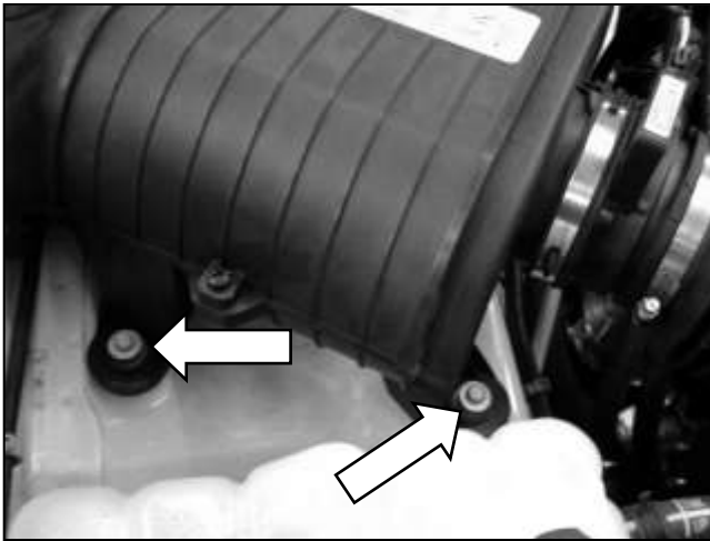
e. Loosen 2 of the bolts holding in the stock air box.
