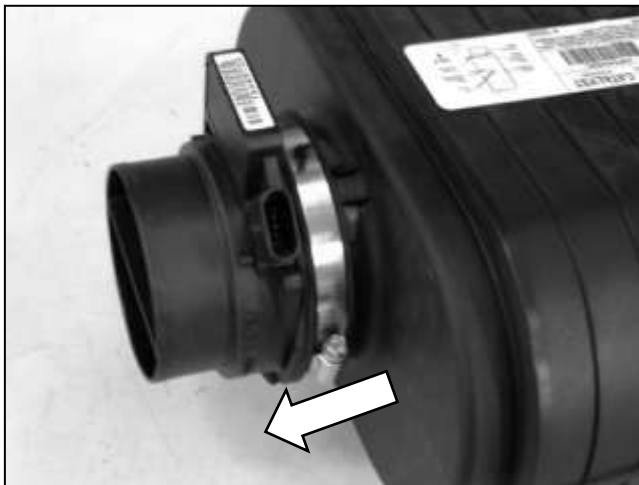
i. Remove the MAF sensor from the stock air box.
