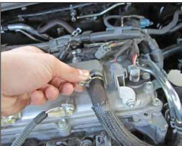
c. Pinch the hose clamp securing the PCV hose to the vent tube on the valve cover, then remove the hose.
