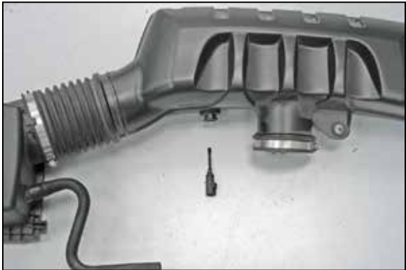
11. Release the locking tab and then remove the inlet air temperature sensor from the factory intake tube by twisting counter clockwise. NOTE: The inlet air temperature sensor is very fragile; take care to avoid damage while handling the sensor.
