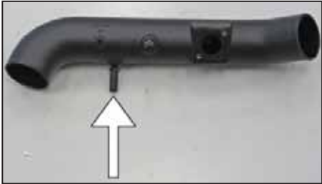
17. Install the provided quick disconnect fitting into the K&N® intake tube as shown.
