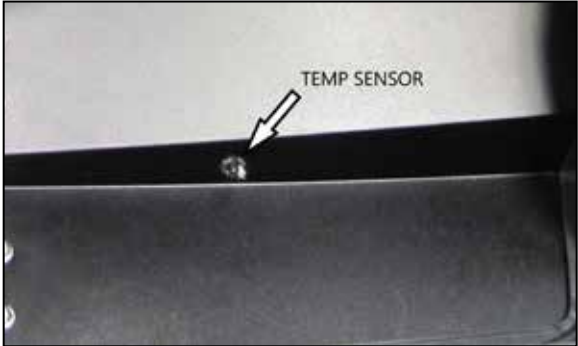
24a. Attach the air temperature sensor from step #23 through the hole on the bottom of the passenger side heat shield on the engine side.
