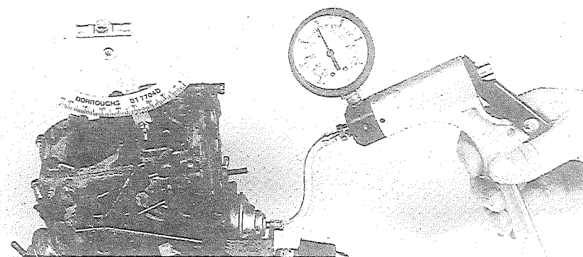
Figure 3.2. Since the late '70s, GM has specified use of a choke angle gauge instead of a pin gauge or drill bit to set choke blade opening. With choke blade closed, set scale to specified choke angle. Apply a vacuum and adjust pull-off until gauge's bubble is centered.
