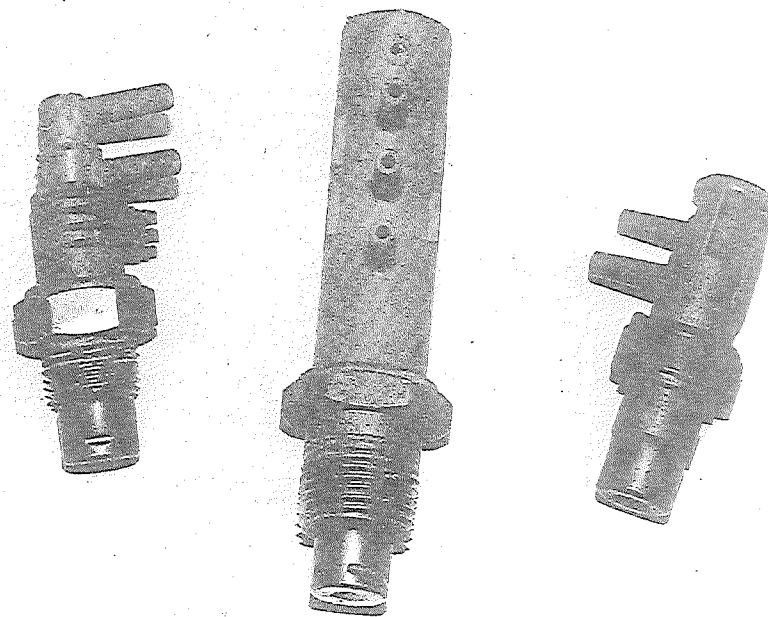
Figure 5.1. Thermal vacuum switches may have many ports or just two. Switches sense coolant temperature, carburetor inlet air temperature, or fuel mixture temperature inside the intake manifold.
