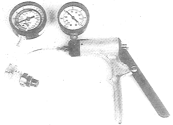
Figure 5.3. This switch is good — it's supposed to pass vacuum when it's cold! When you suspect a switch is popping open at the wrong time, tee a vacuum gauge into its circuit. Road test the car hot and cold and watch the vacuum gauge.
