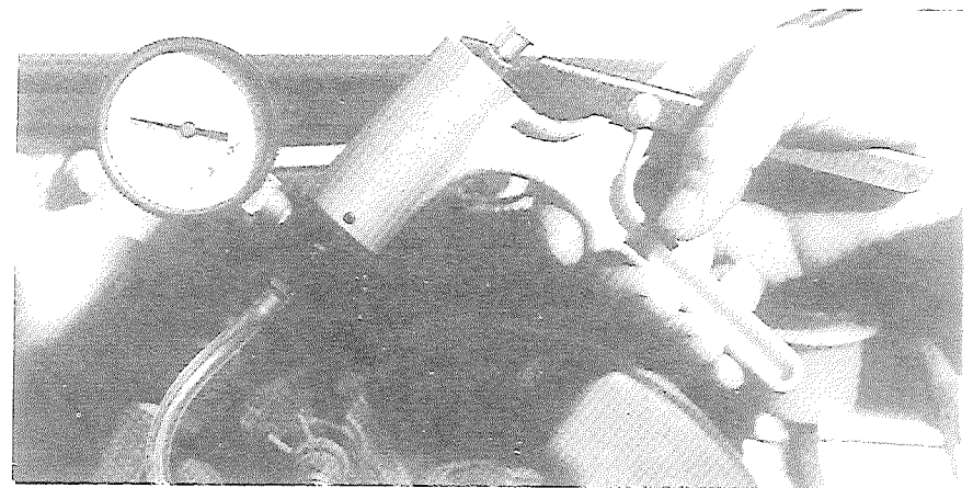
Figure 7.1. Poor-running engine with low manifold vacuum can affect power booster operation. Leaking power booster check valve is common condition. Always retest the booster after you've replaced a check valve.
