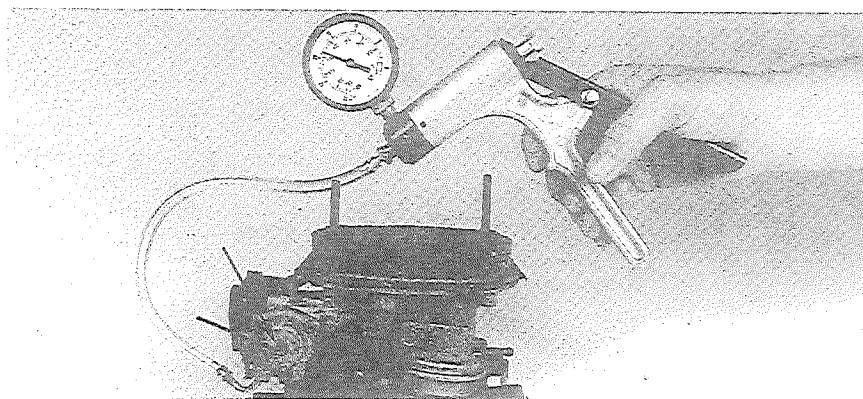
Figure 3.3. On this Holley/Chrysler carb, apply a vacuum to the pull-off and then turn the set screw (arrow) until the specified-size drill fits between the top of the choke blade and the air horn wall.
