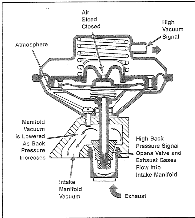
Figure 5.14. Here is one type of integral backpressure EGR valve. Unless exhaust backpressure is present — unless the engine is running — the air bleed in the center of the valve will remain open. You cannot pump open this EGR valve when the engine's not running. Check your manual for the specifications of the unit you are testing.
