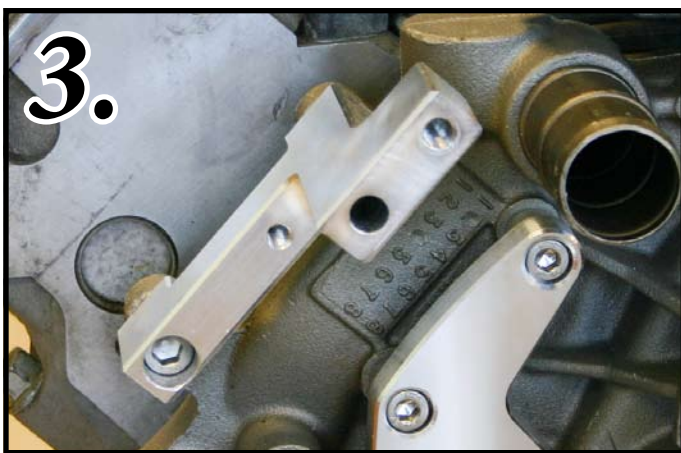
Photo 3: Install Rear A/C Bracket (20067-B) to the water pump as shown using one 10mm x 30mm SHCS (S561) bolt in the lower mounting hole. Snug only at this time.
