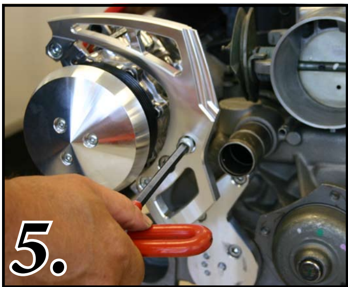
Photo 5: Place one \frac{3}{8} - 16 x 1" SHCS (S248) into upper hole and secure Main A/C bracket to the Rear A/C Bracket.
