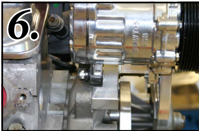
Photo 6: Bolt the A/C rear mounting ear to Rear A/C Bracket using one \frac{5}{16} " x 1\frac{1}{2} " SHCS (S150)
