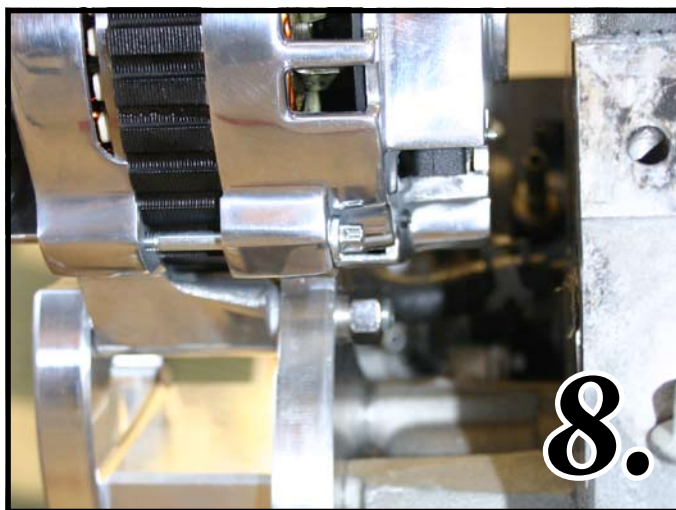
Photo 8: Install Alternator (P571) using one \frac{3}{8} -16 x 3\frac{1}{4} " SHCS (S268) thru front main bracket and rear bushing secure with one \frac{3}{8} " Locknut (S622). Secure the top alternator mount using one 8mm x 25mm SHCS (S551) SHCS.
