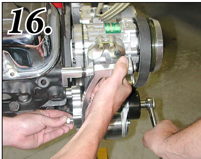
Photo-16 INSTALLING THE BELT
