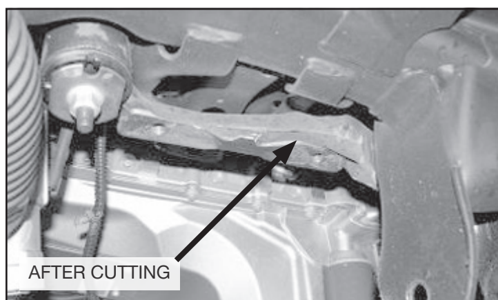
FIGURE 21 - STEP 17
