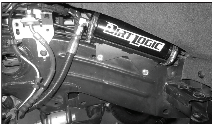
FIGURE 6 - STEP 4
