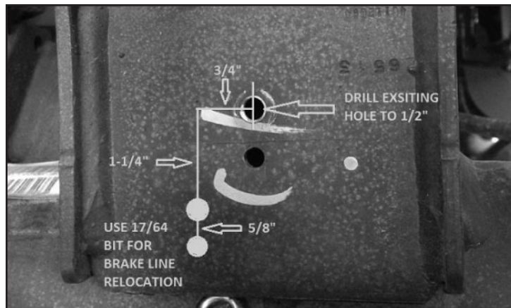
FIGURE 65 - STEP 55
