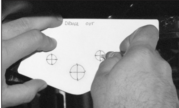
FIGURE 32 - STEP 37
