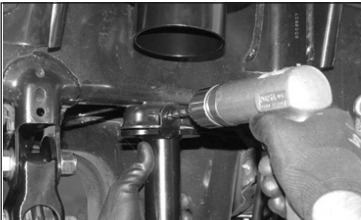
FIGURE 25 - STEP 29
