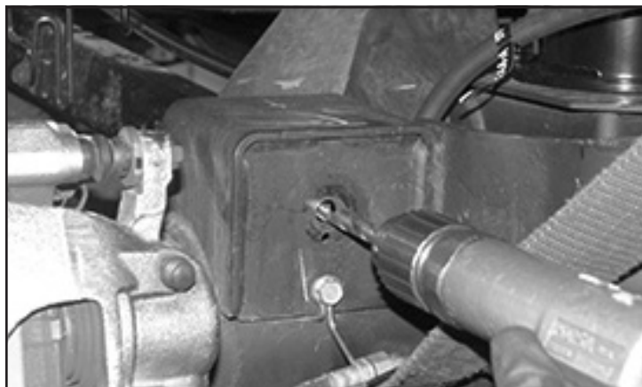
FIGURE 66 - STEP 56
