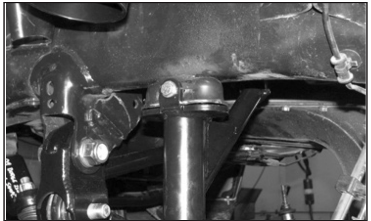
FIGURE 26 - STEP 30
