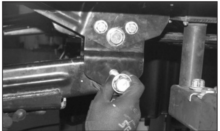
FIGURE 46 - STEP 44
