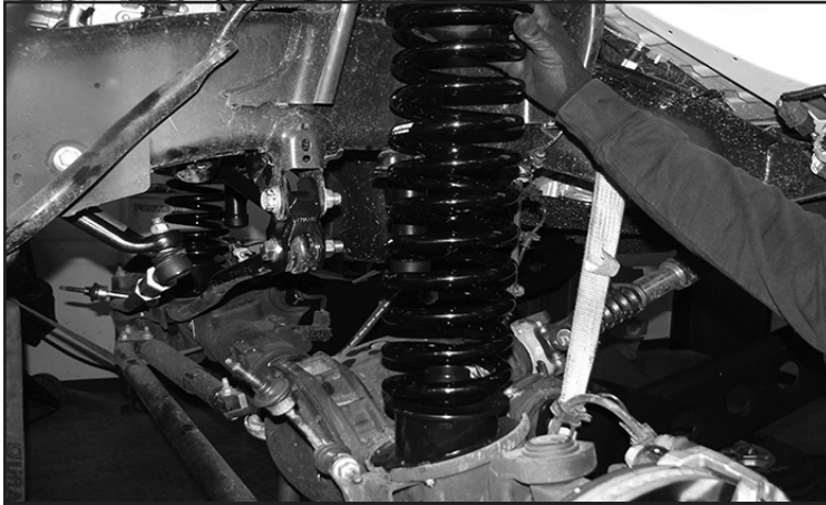
FIGURE 53 - STEP 49
