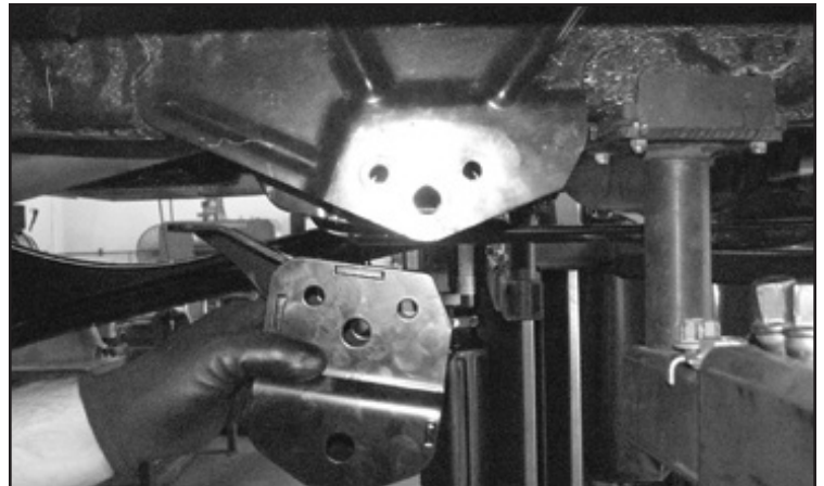
FIGURE 33 - STEP 40
