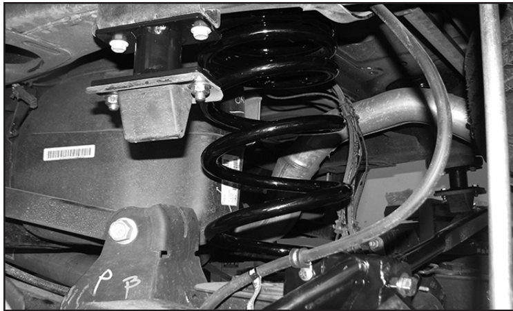
FIGURE 76 - STEP 68
