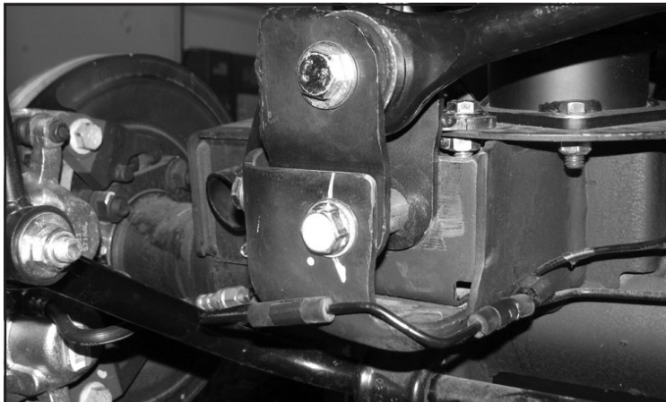
FIGURE 77 - STEP 69
