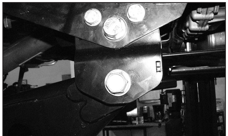
FIGURE 46 - STEP 47
