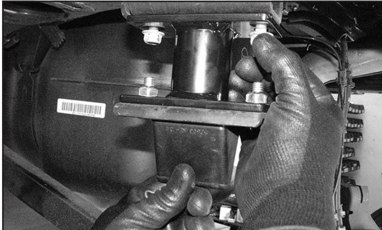
FIGURE 75 - STEP 67
