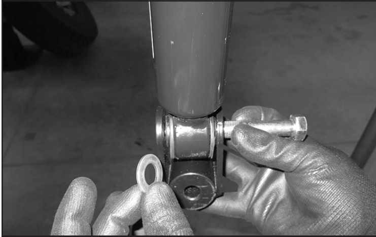
FIGURE 6 - STEP 5
