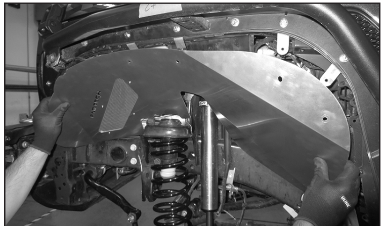
FIGURE 10 - STEP 9
