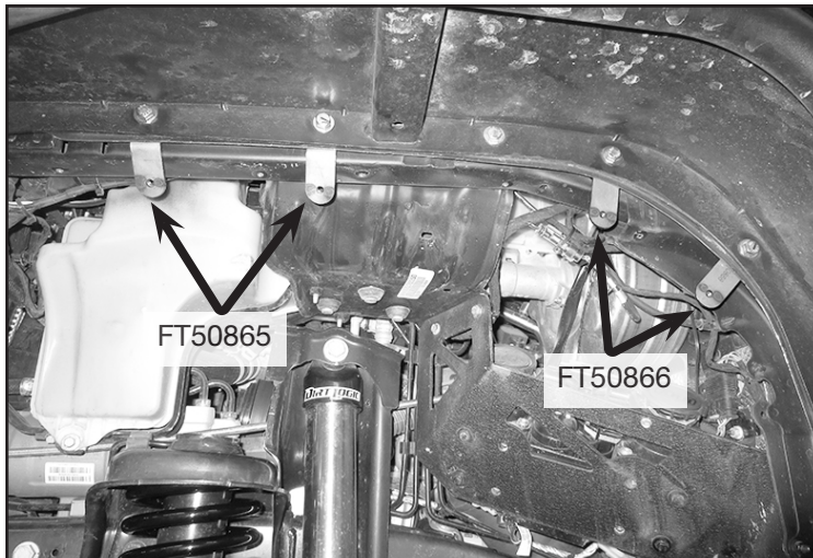
FIGURE 7 - STEP 6
