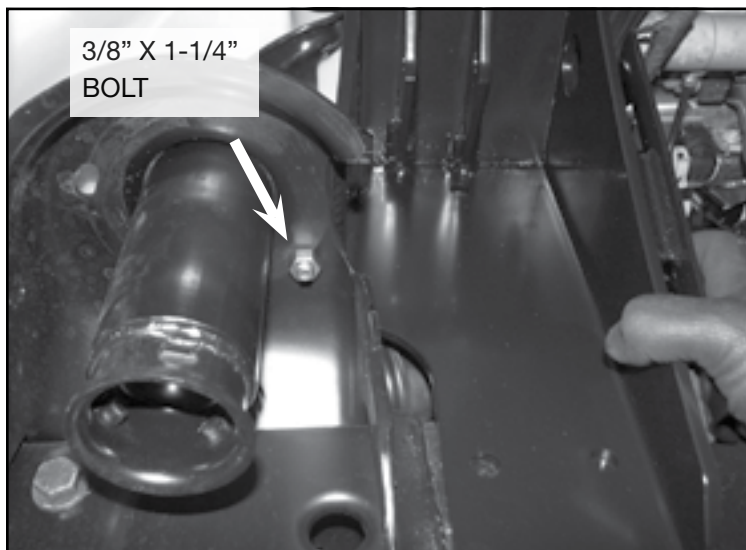
FIGURE 12 - STEP 11
