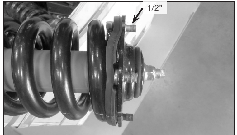
FIGURE 7 - STEP 12
