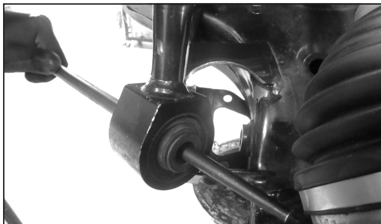
FIGURE 11 - STEP 15
