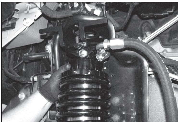
FIGURE 15 - STEP 18
