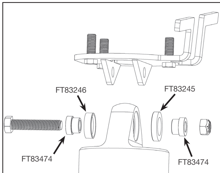
FIGURE 11 - STEP 14
