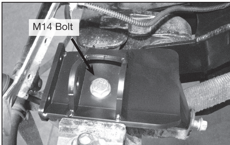
FIGURE 13 - STEP 16
