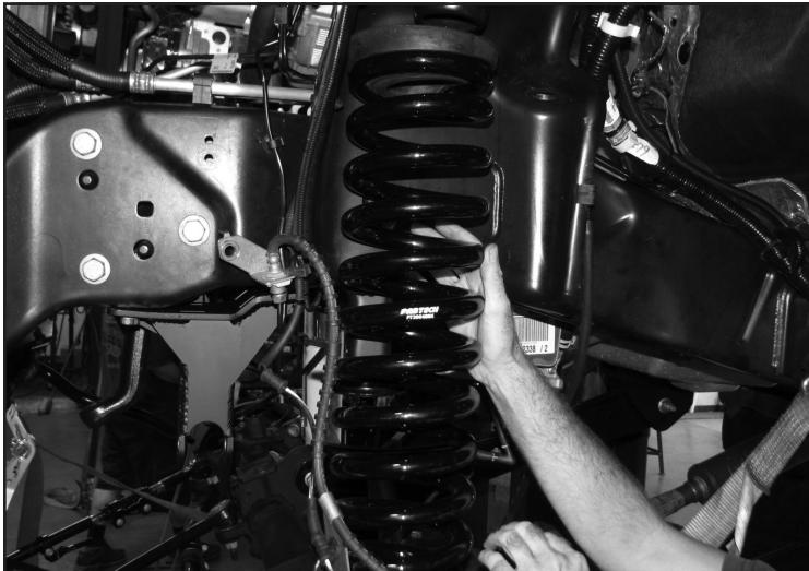
FIGURE 24 - STEP 23
