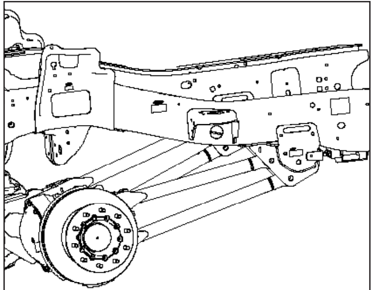
FIGURE 22 - STEP 22
