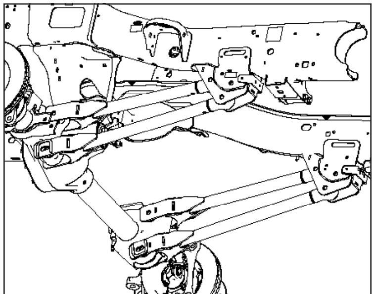
FIGURE 23 - STEP 22
