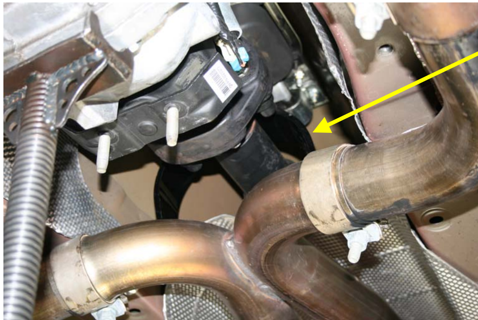
Step 5: Place drive shaft loop around drive shaft
