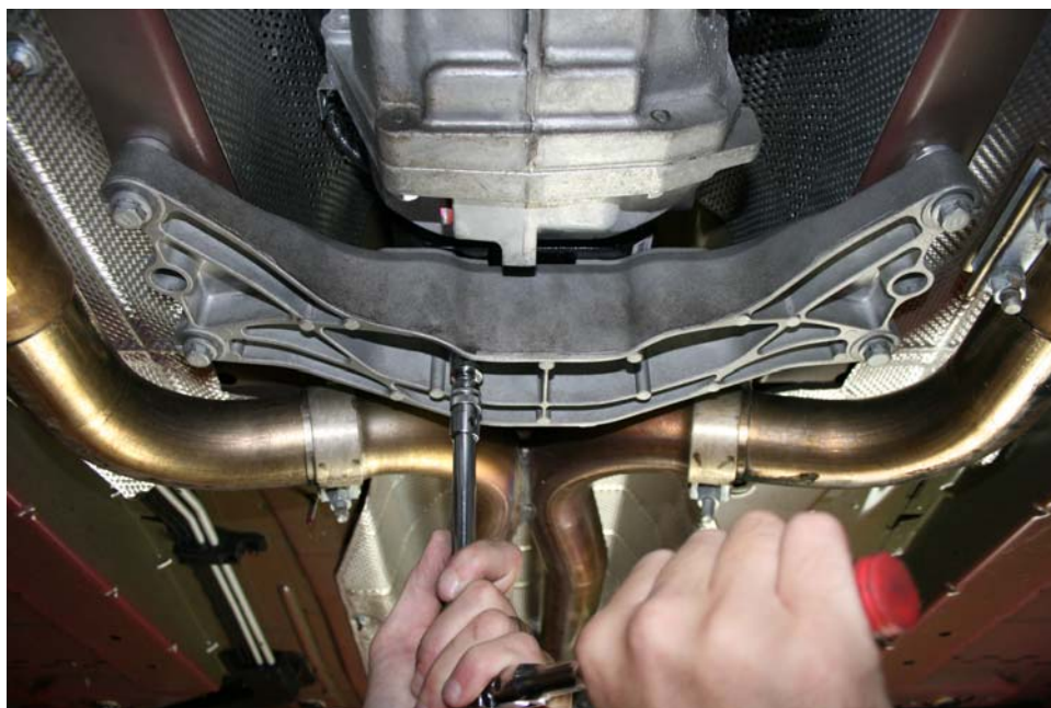
Step 11: Reinstall and tighten transmission mount bolts
