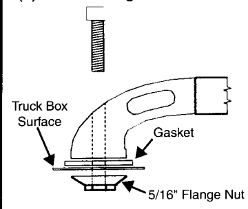
(C) For Mounting With Toolbox
