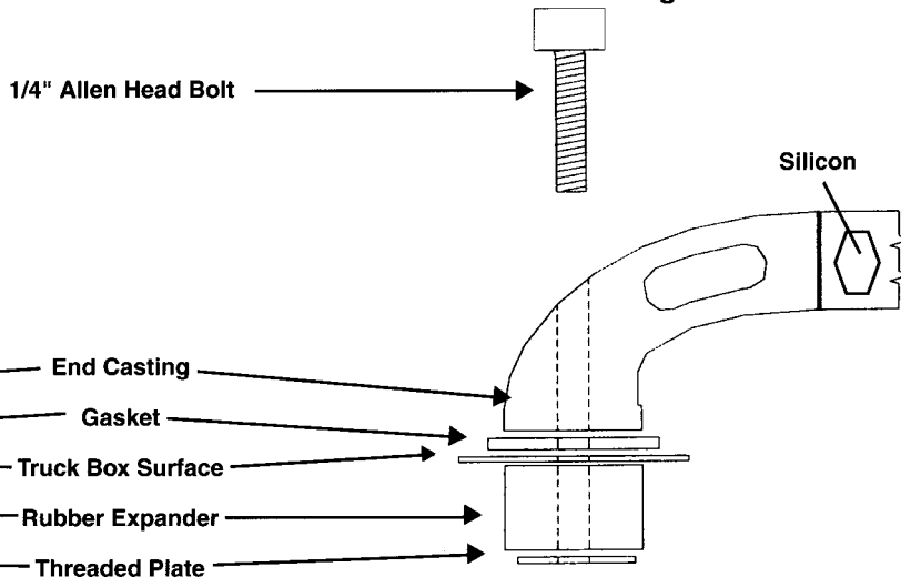
(B) For Mounting to Sidebed When Not Using Stake Pocket
