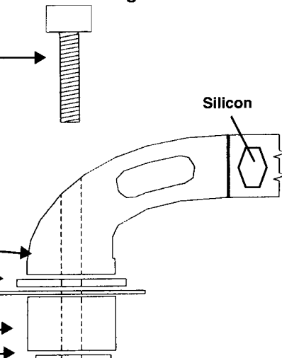
(B) For Mounting to Sidebed When Not Using Stake Pocket
