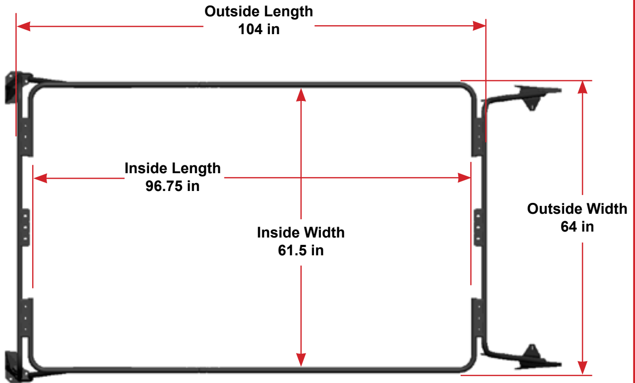
JK / JL Base Rack Dimensions
