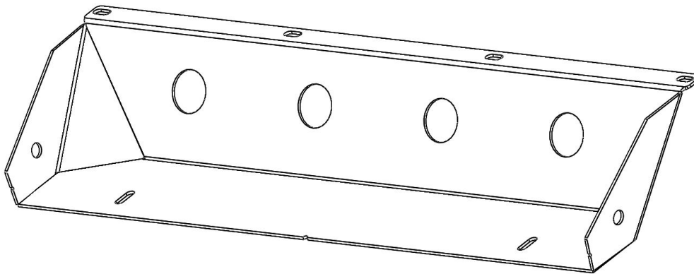
DESTROYER SKID PLATE 4JSP1800-01 (x1)
