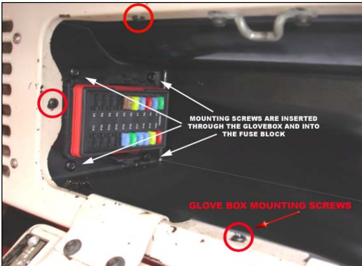
FUSE BLOCK MOUNTING 2
