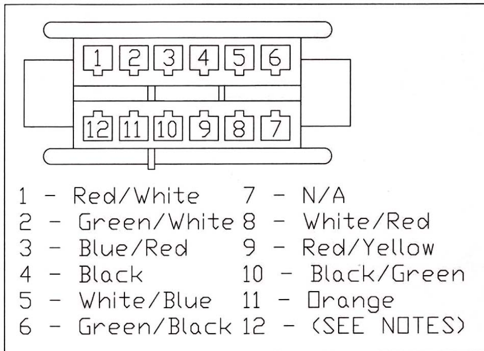
Figure 7-37 1972 Cluster Pigtail Pinout (If 18 Pin Connector use Figure 7-36)
