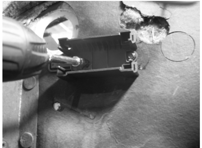
Figure 6-3 Fuse Block Base Position '73-'77
