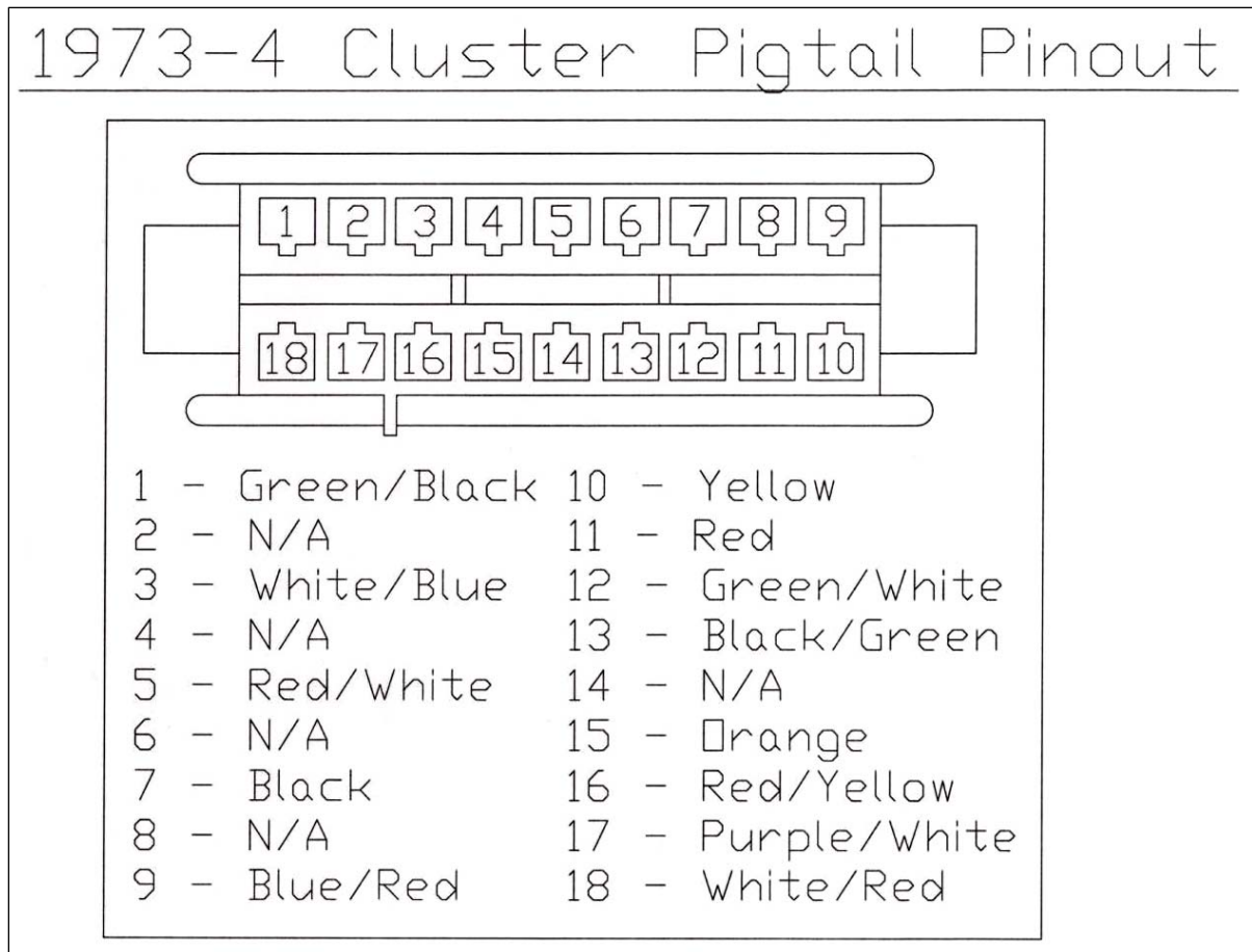
Figure 7-38 1973 - 1974 Cluster Pigtail Pinout
