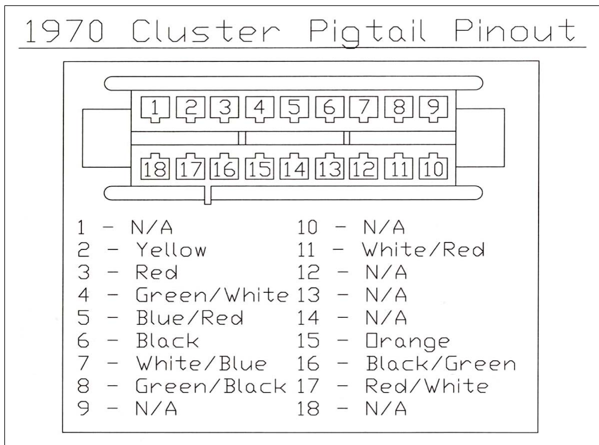
Figure 7-35 1970 Cluster Pigtail Pinout
