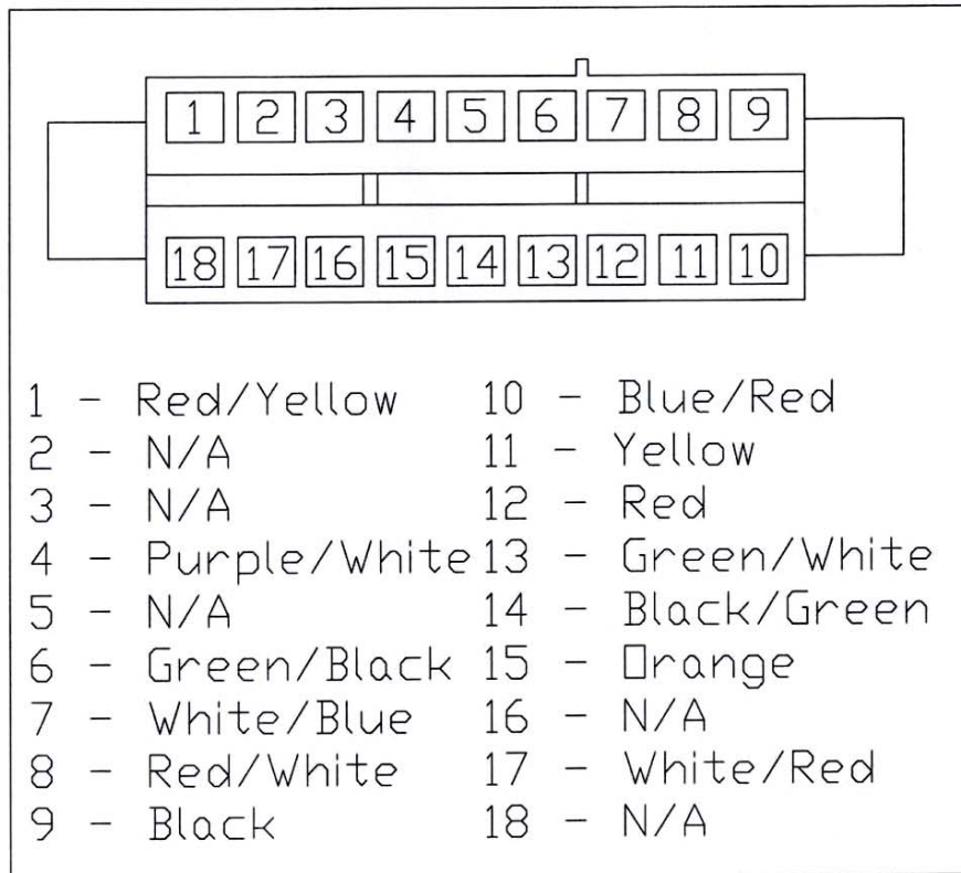
Figure 7-40 1976-77 Cluster Pigtail Pinout
