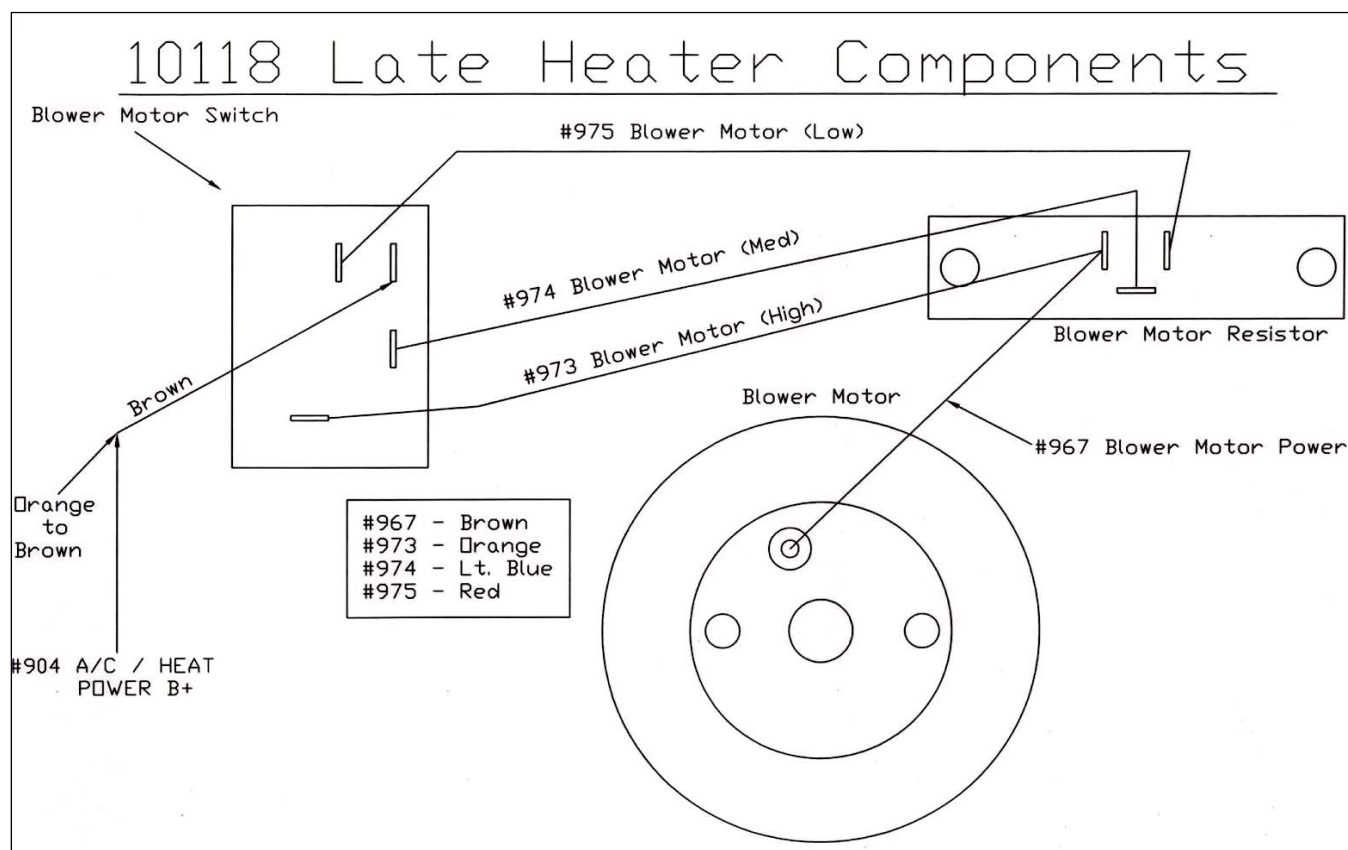
Figure 7-30 Heater Harness Installation for 1973-1977 years only.
